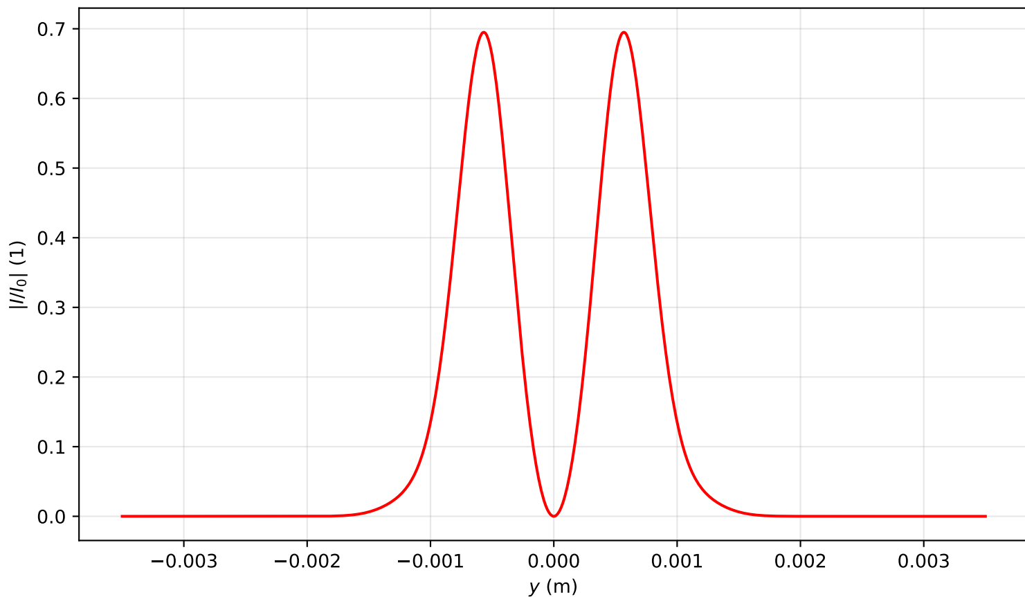
Intensity profile I(x=0, y, z=0.876)/I_0 , \text{Pin}=2.0\text{Pcr} , artificial time
